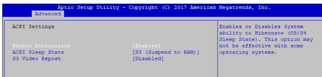
Figure 4-3-5: ACPI Settings
