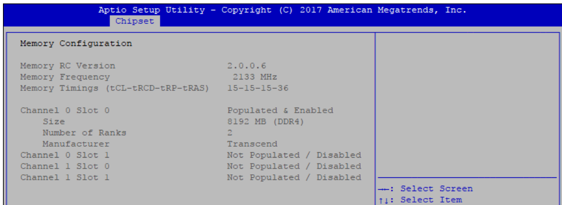
Figure 4-4-1-1: Memory Configuration
