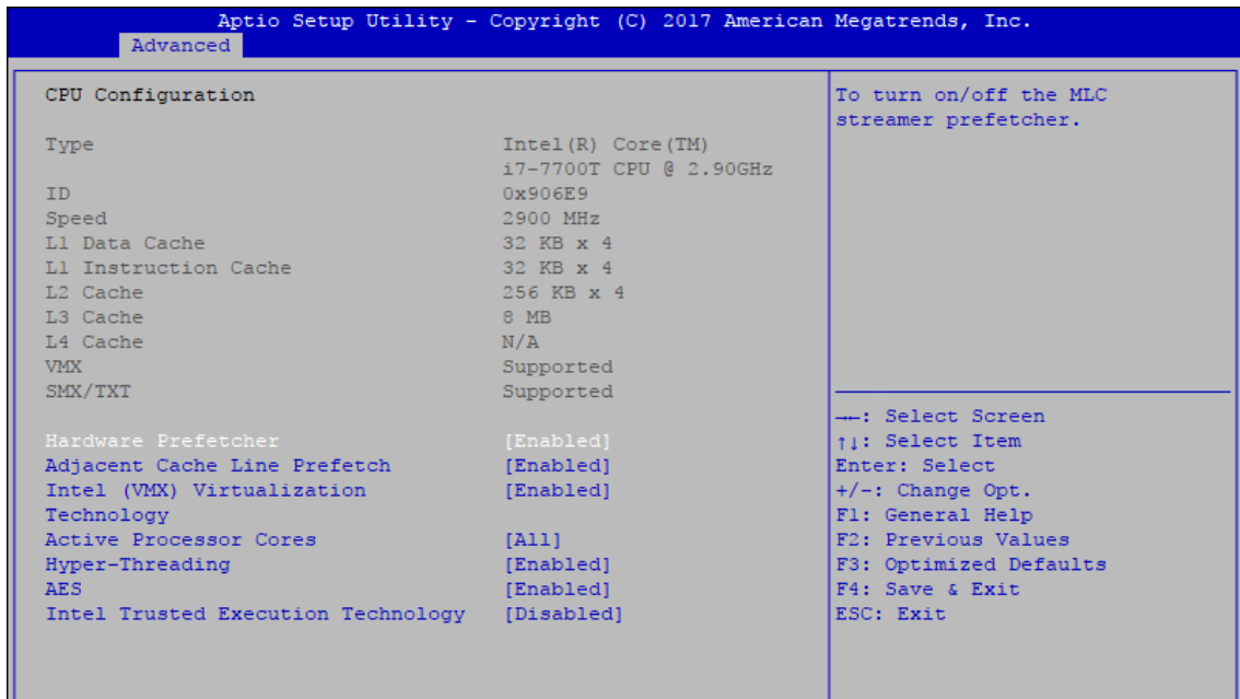
Figure 4-3-1: CPU Configuration
