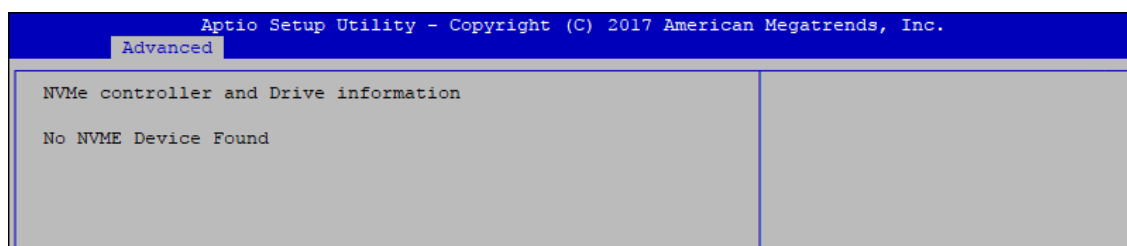
Figure 4-3-15: NVMe Configuration
