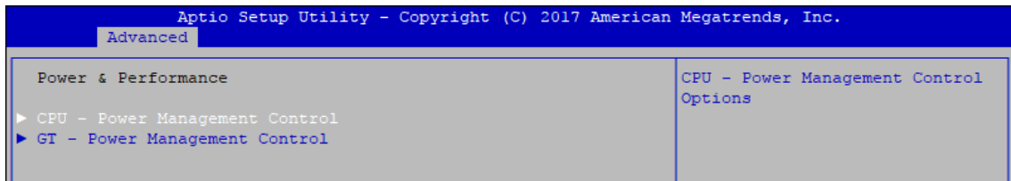
Figure 4-3-2: Power & Performance
