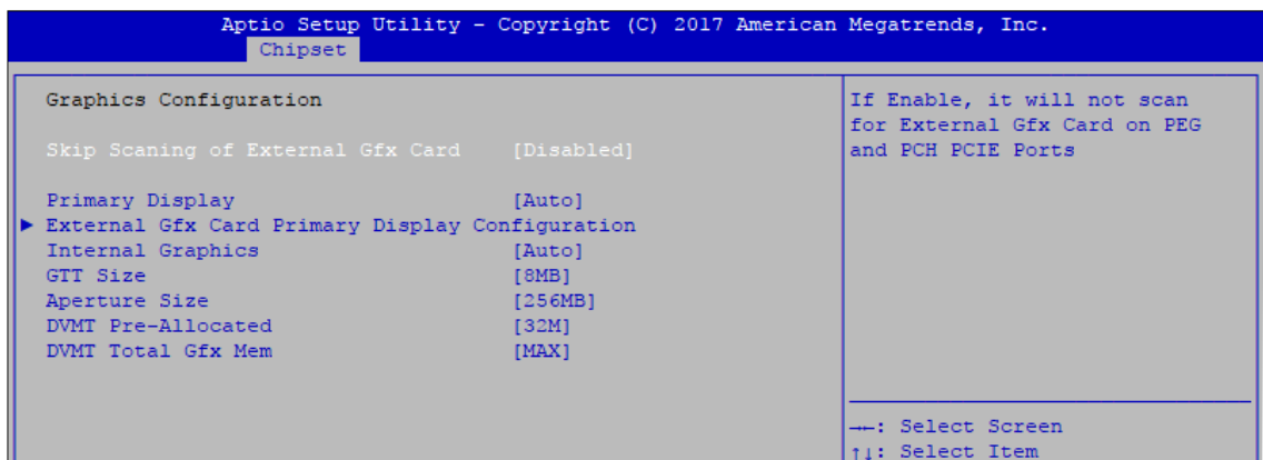
Figure 4-4-1-2: Graphics Configuration
