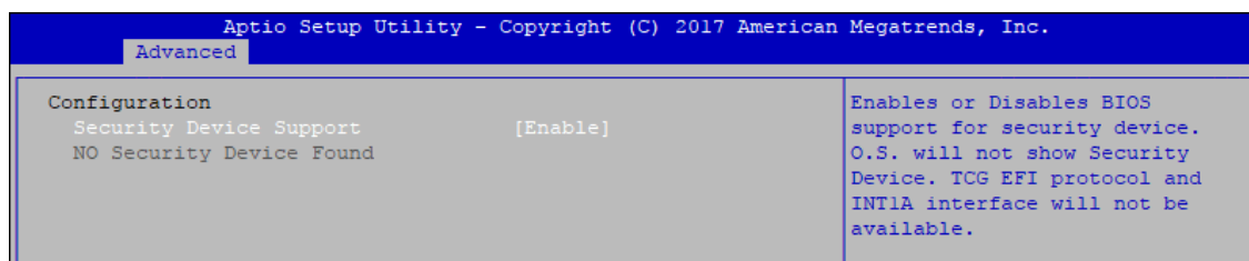
Figure 4-3-4: Trusted Computing
