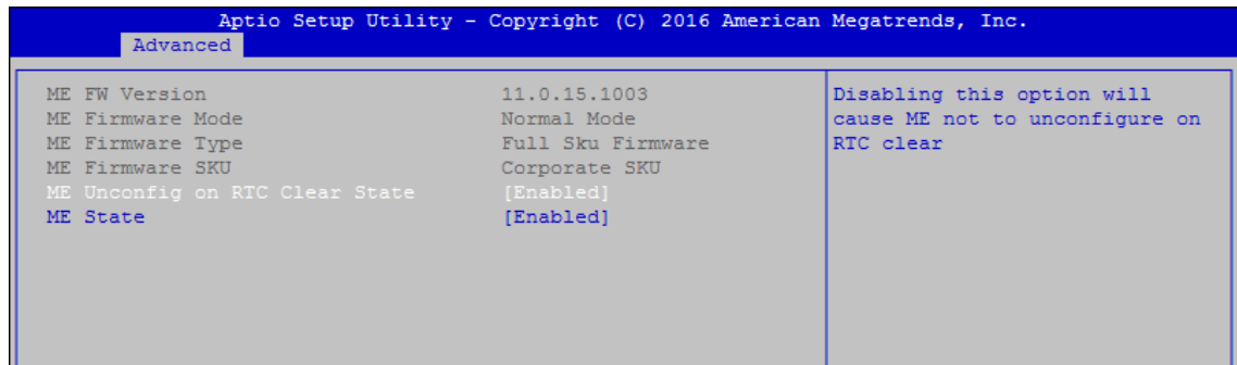
Figure 4 3-3: PCH-FW Settings
