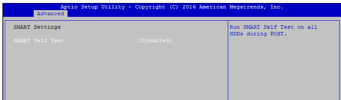
Figure 4 3-4: SMART Settings
